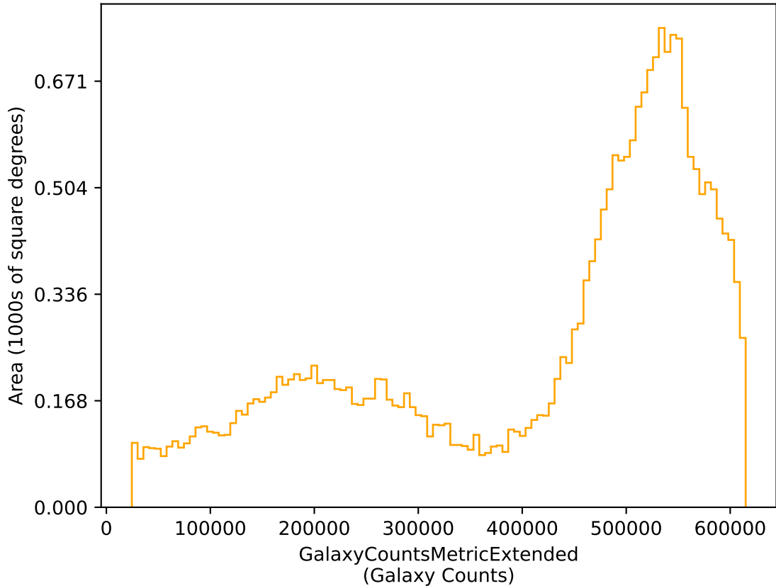
too_elab_r256_d2_ugrizy_v3.4_10yrs r: GalaxyCountsMetricExtended
