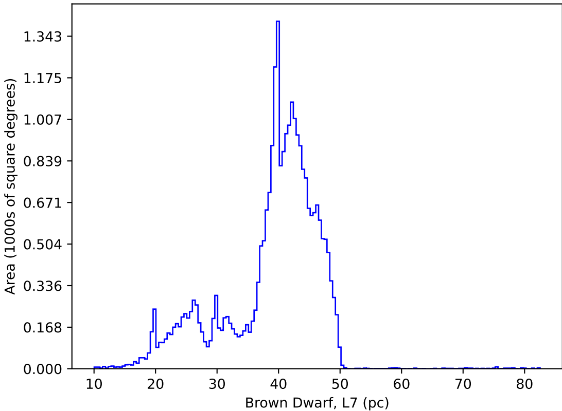
too_elab_r256_d2_ugrizy_v3.4_10yrs : Brown Dwarf, L7
