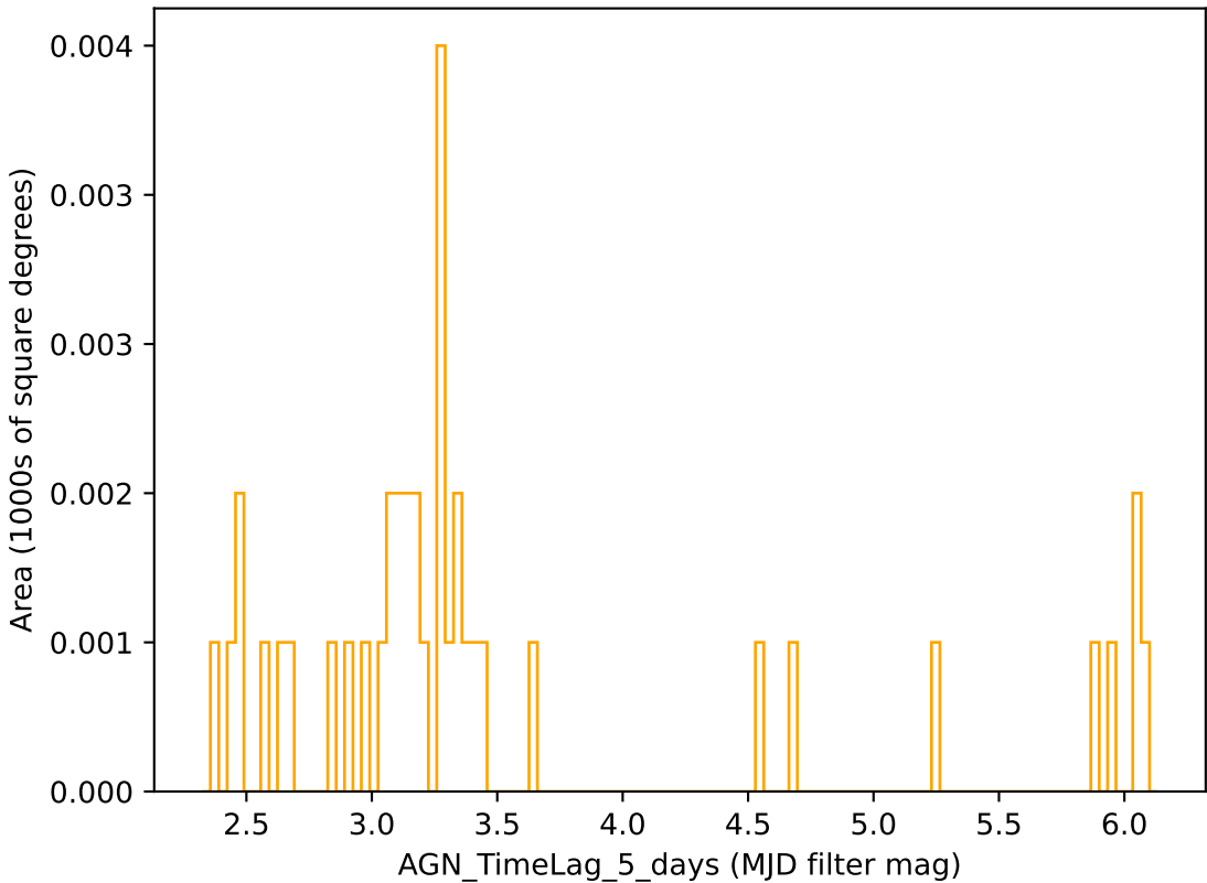
too_elab_r256_d2_ugrizy_v3.4_10yrs r band: AGN_TimeLag_5_days
