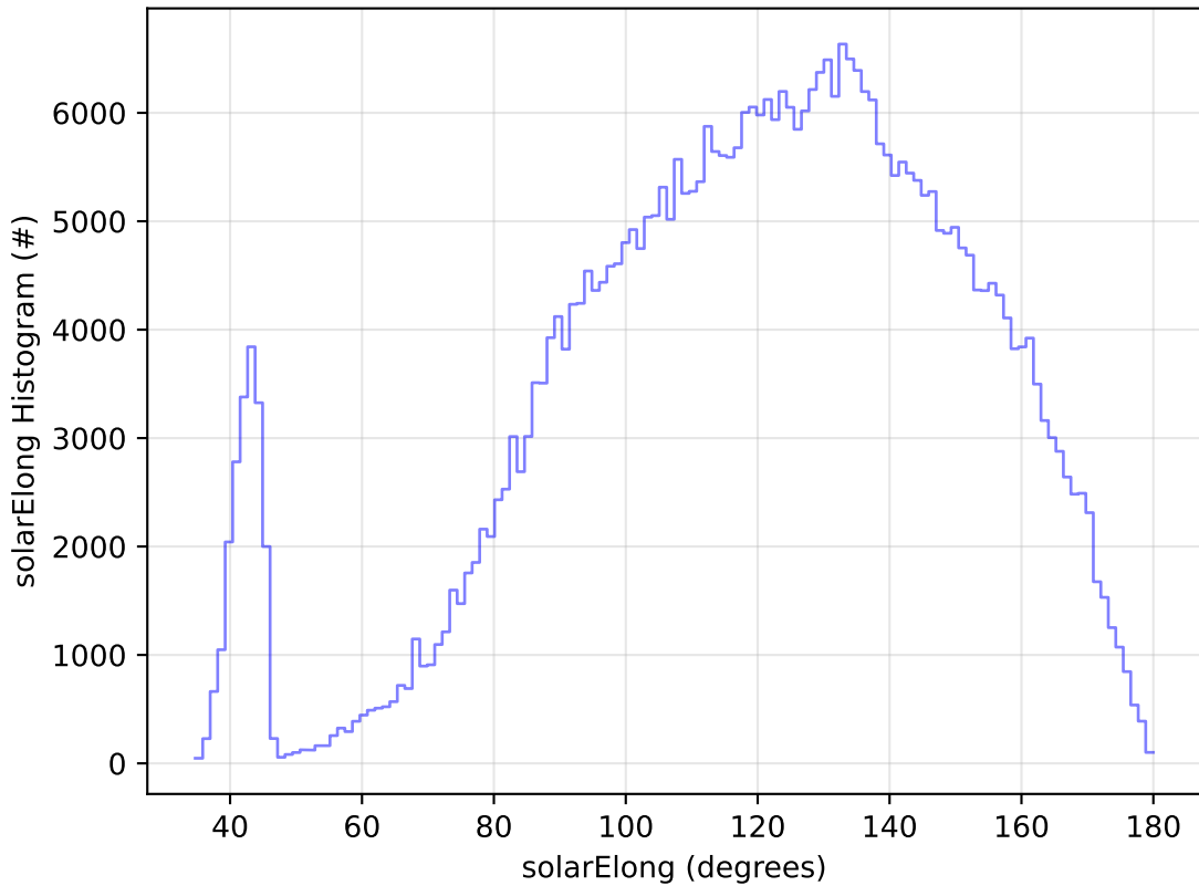
too_elab_r256_d2_ugrizy_v3.4_10yrs WFD z band: solarElong Histogram
