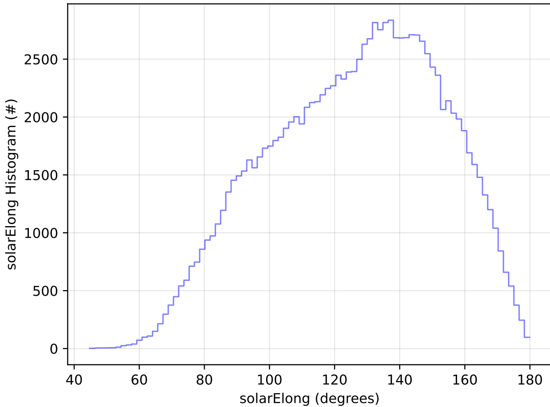
too_elab_r256_d2_ugrizy_v3.4_10yrs WFD u band: solarElong Histogram
