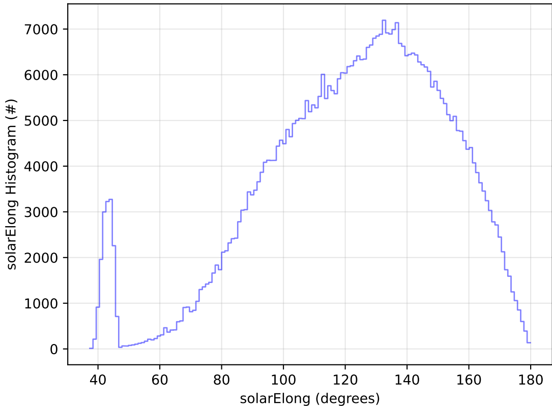
too_elab_r256_d2_ugrizy_v3.4_10yrs WFD r band: solarElong Histogram
