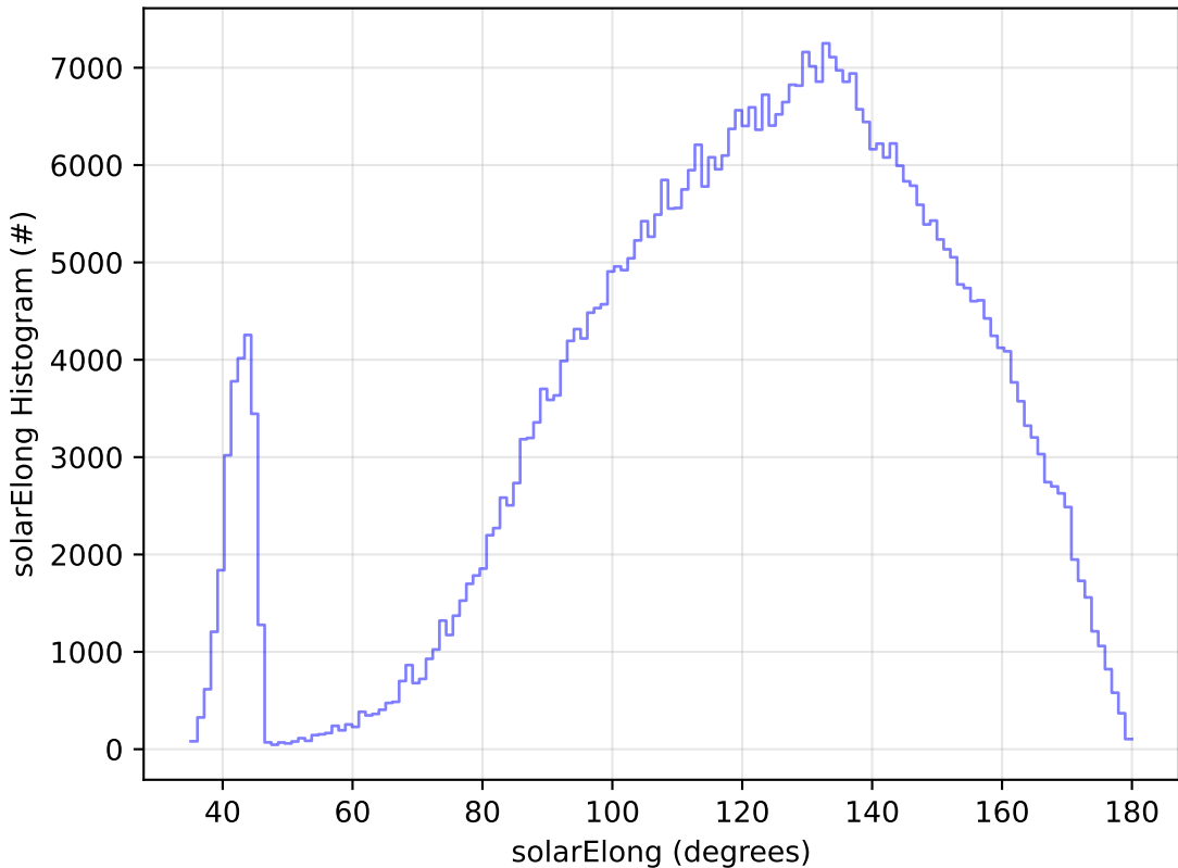
too_elab_r256_d2_ugrizy_v3.4_10yrs WFD i band: solarElong Histogram
