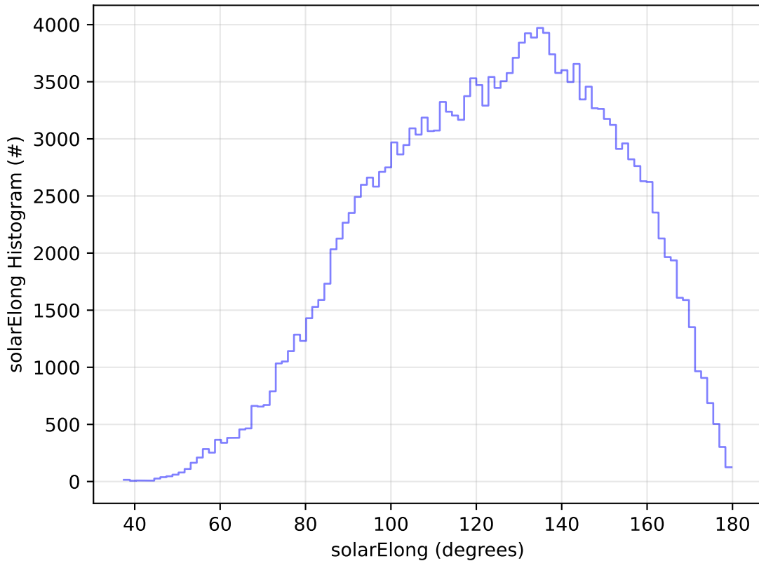
too_elab_r256_d2_ugrizy_v3.4_10yrs WFD g band: solarElong Histogram
