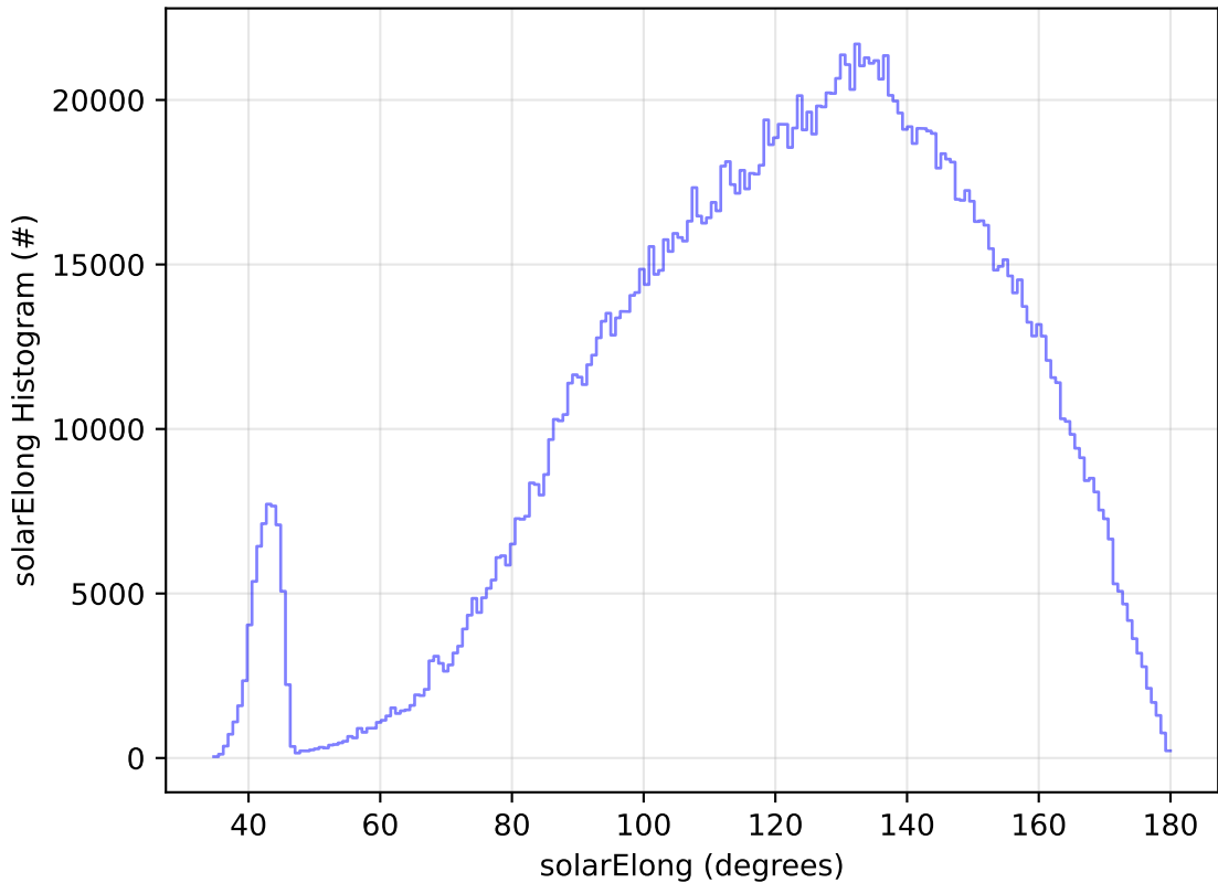
too_elab_r256_d2_ugrizy_v3.4_10yrs WFD all bands: solarElong Histogram
