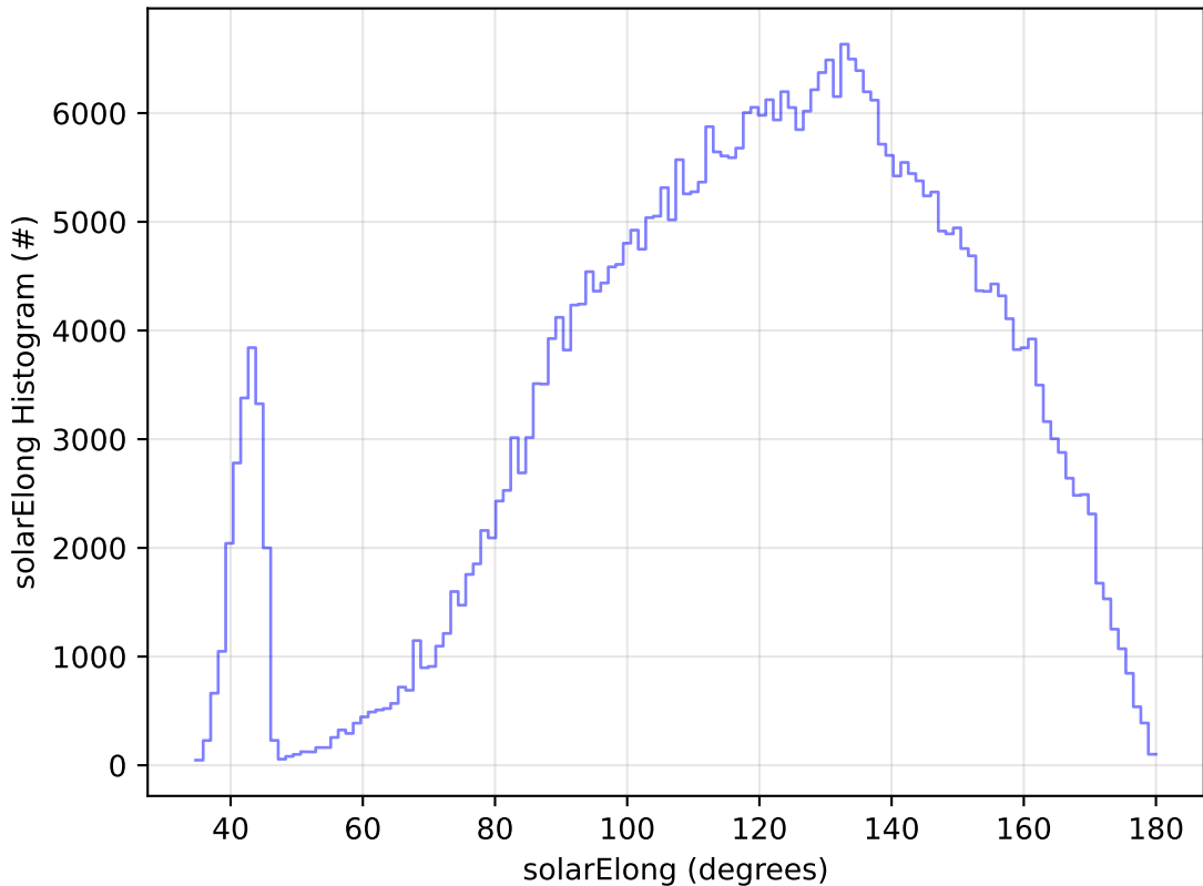
too_elab_r256_d2_ugrizy_v3.4_10yrs All sky z band: solarElong Histogram
