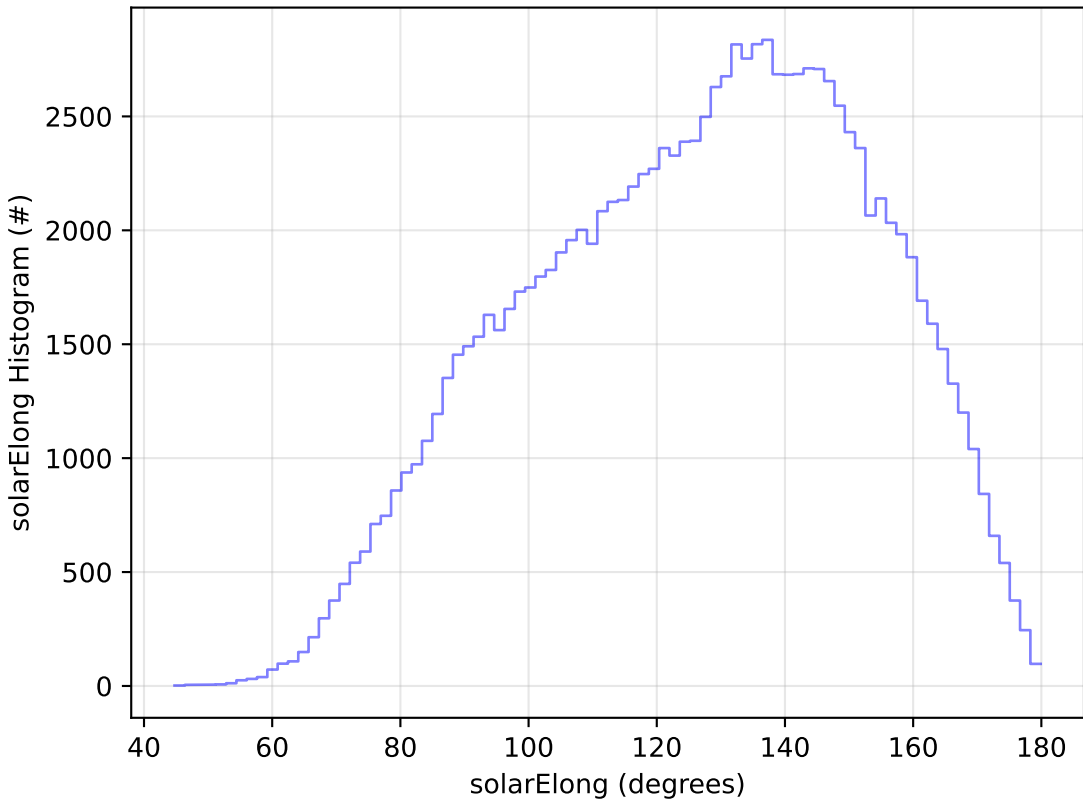
too_elab_r256_d2_ugrizy_v3.4_10yrs All sky u band: solarElong Histogram
