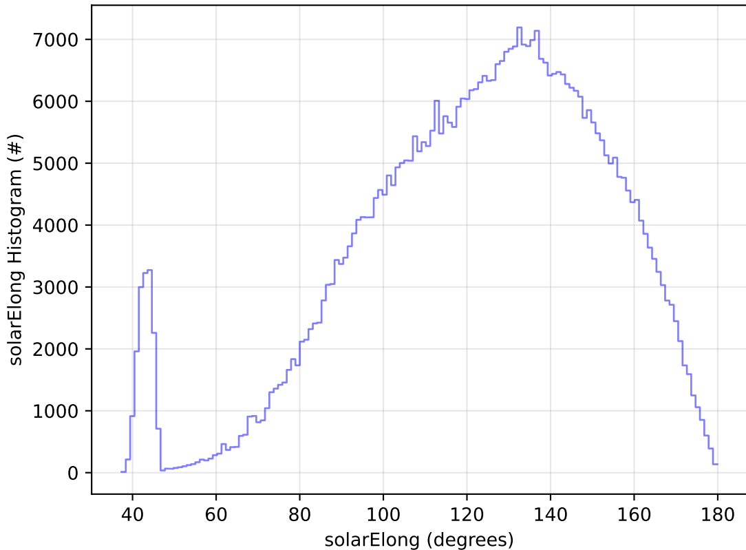
too_elab_r256_d2_ugrizy_v3.4_10yrs All sky r band: solarElong Histogram
