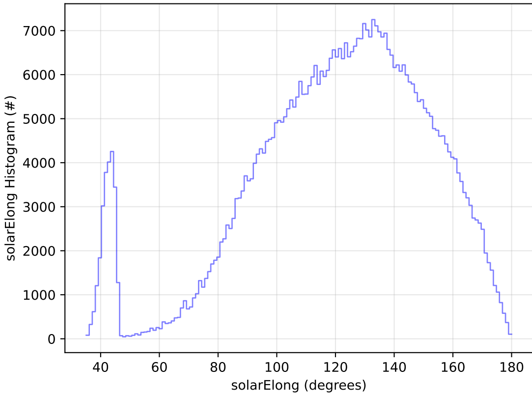
too_elab_r256_d2_ugrizy_v3.4_10yrs All sky i band: solarElong Histogram
