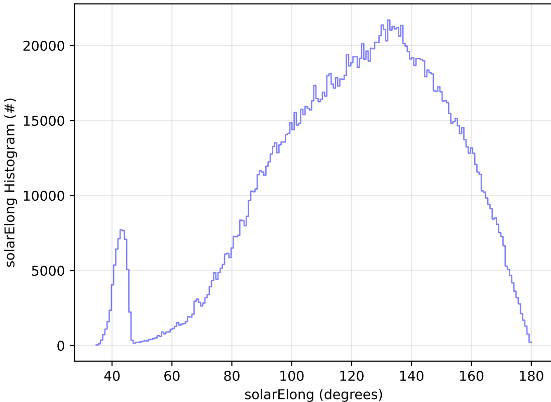
too_elab_r256_d2_ugrizy_v3.4_10yrs All sky all bands: solarElong Histogram
