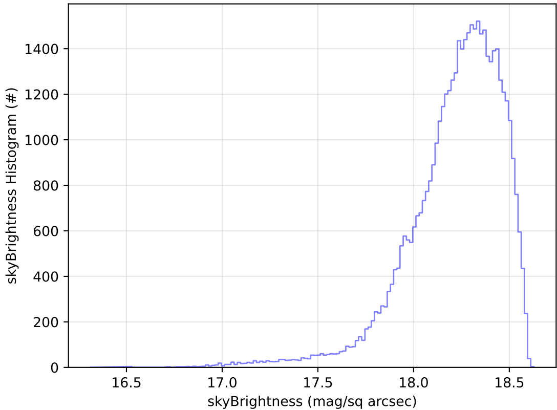
too_elab_r256_d2_ugrizy_v3.4_10yrs Yr 1 y band: skyBrightness Histogram
