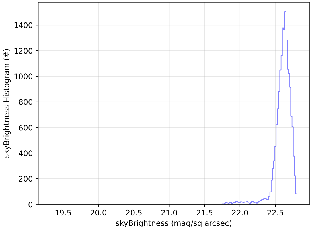
too_elab_r256_d2_ugrizy_v3.4_10yrs Yr 1 u band: skyBrightness Histogram
