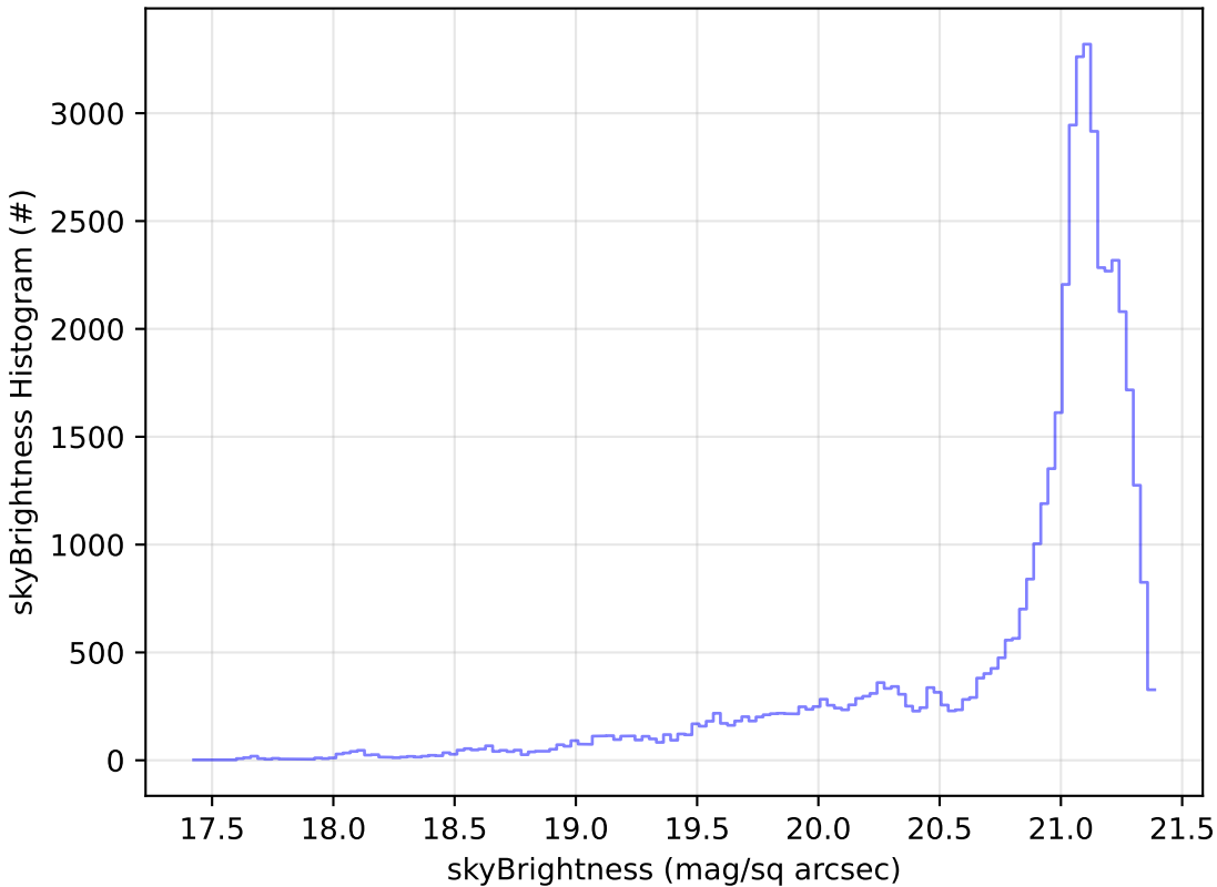
too_elab_r256_d2_ugrizy_v3.4_10yrs Yr 1 r band: skyBrightness Histogram
