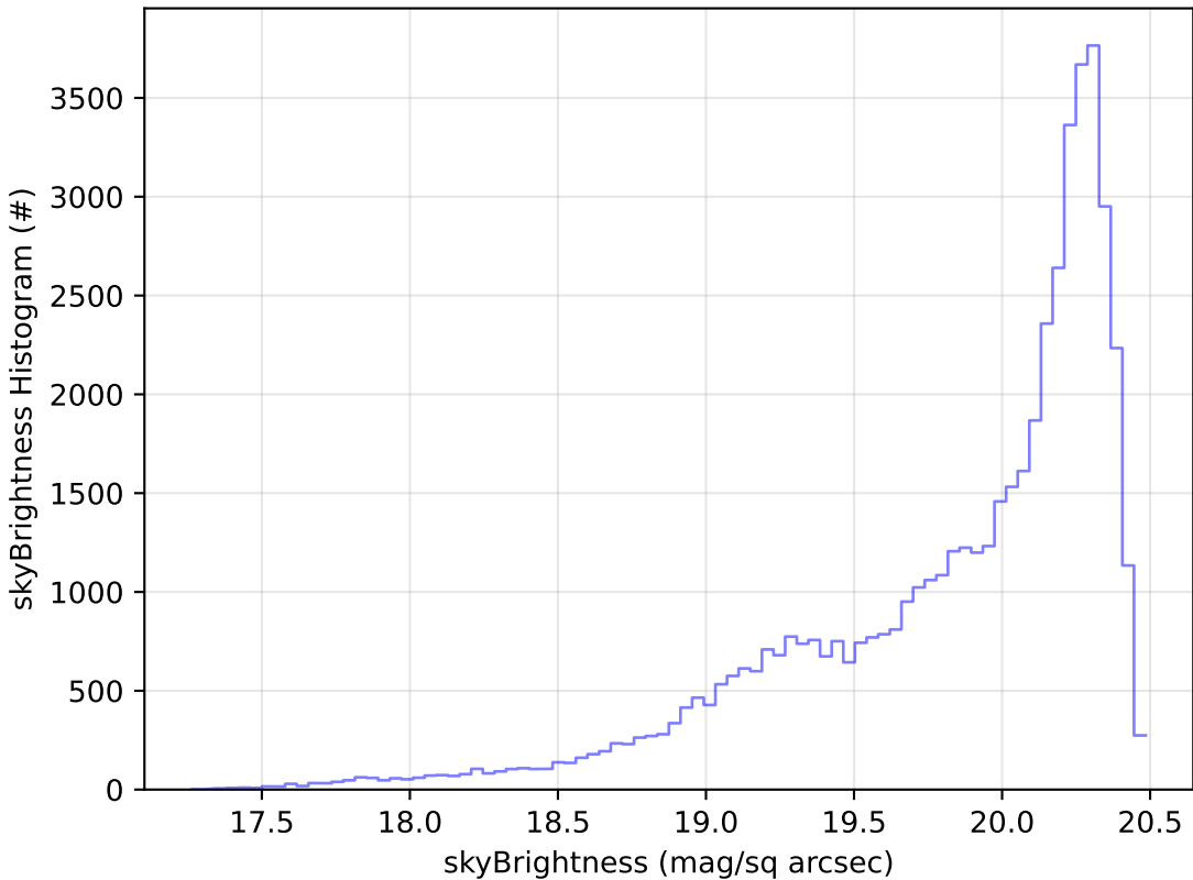
too_elab_r256_d2_ugrizy_v3.4_10yrs Yr 1 i band: skyBrightness Histogram
