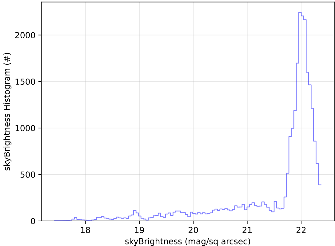
too_elab_r256_d2_ugrizy_v3.4_10yrs Yr 1 g band: skyBrightness Histogram
