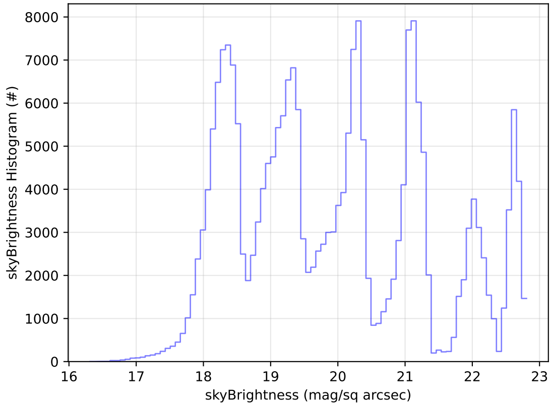
too_elab_r256_d2_ugrizy_v3.4_10yrs Yr 1 all bands: skyBrightness Histogram
