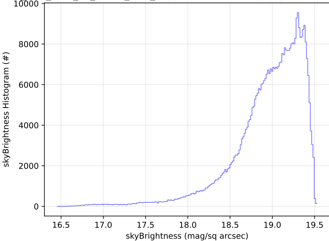
too_elab_r256_d2_ugrizy_v3.4_10yrs WFD z band: skyBrightness Histogram
