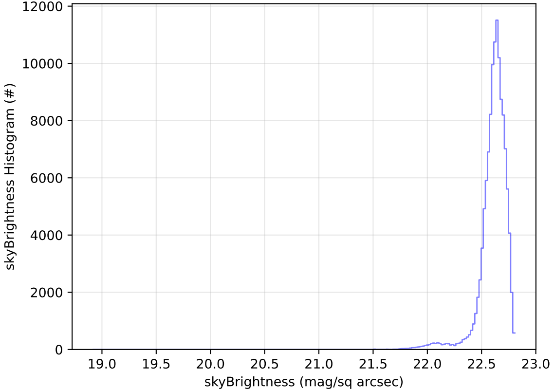
too_elab_r256_d2_ugrizy_v3.4_10yrs WFD u band: skyBrightness Histogram
