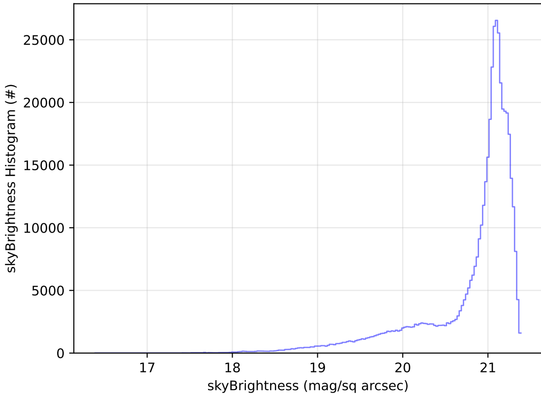
too_elab_r256_d2_ugrizy_v3.4_10yrs WFD r band: skyBrightness Histogram
