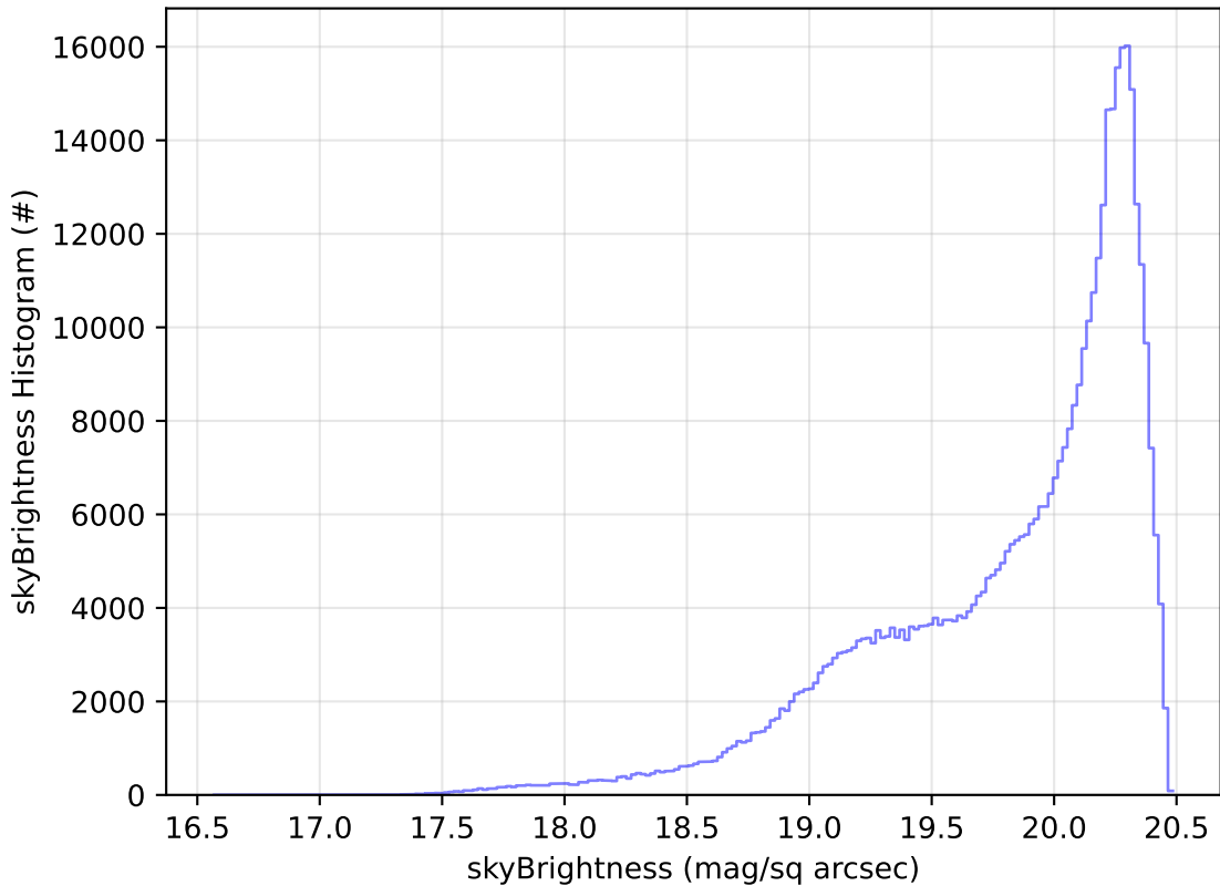
too_elab_r256_d2_ugrizy_v3.4_10yrs WFD i band: skyBrightness Histogram
