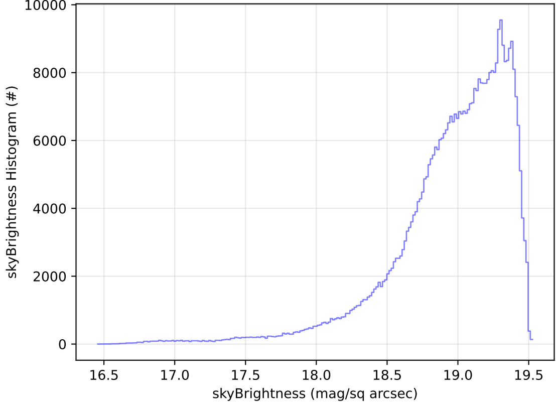
too_elab_r256_d2_ugrizy_v3.4_10yrs All sky z band: skyBrightness Histogram
