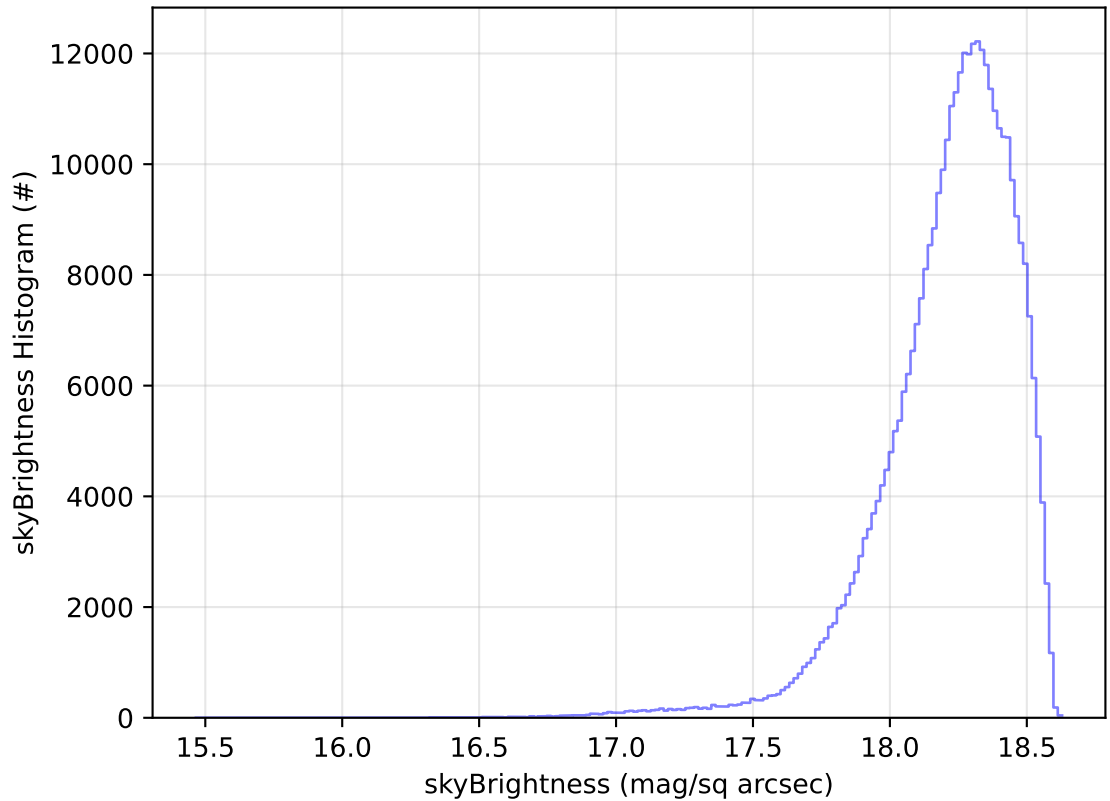
too_elab_r256_d2_ugrizy_v3.4_10yrs All sky y band: skyBrightness Histogram
