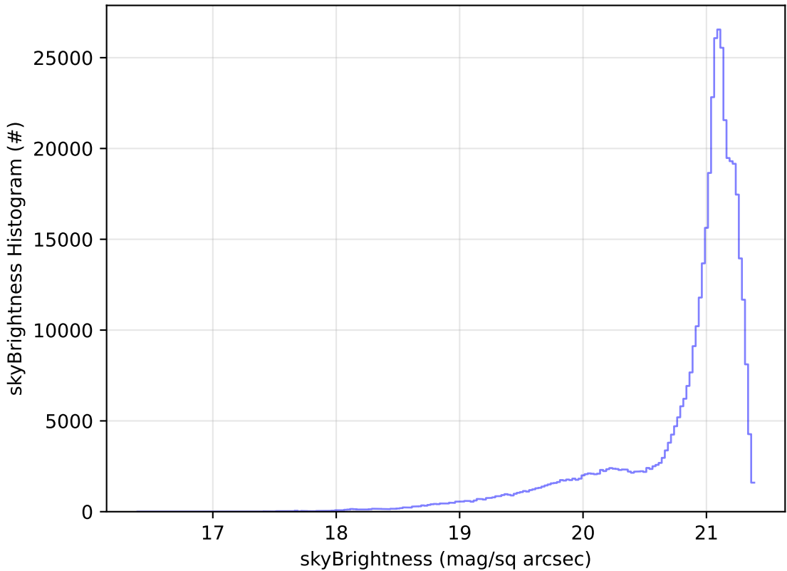
too_elab_r256_d2_ugrizy_v3.4_10yrs All sky r band: skyBrightness Histogram
