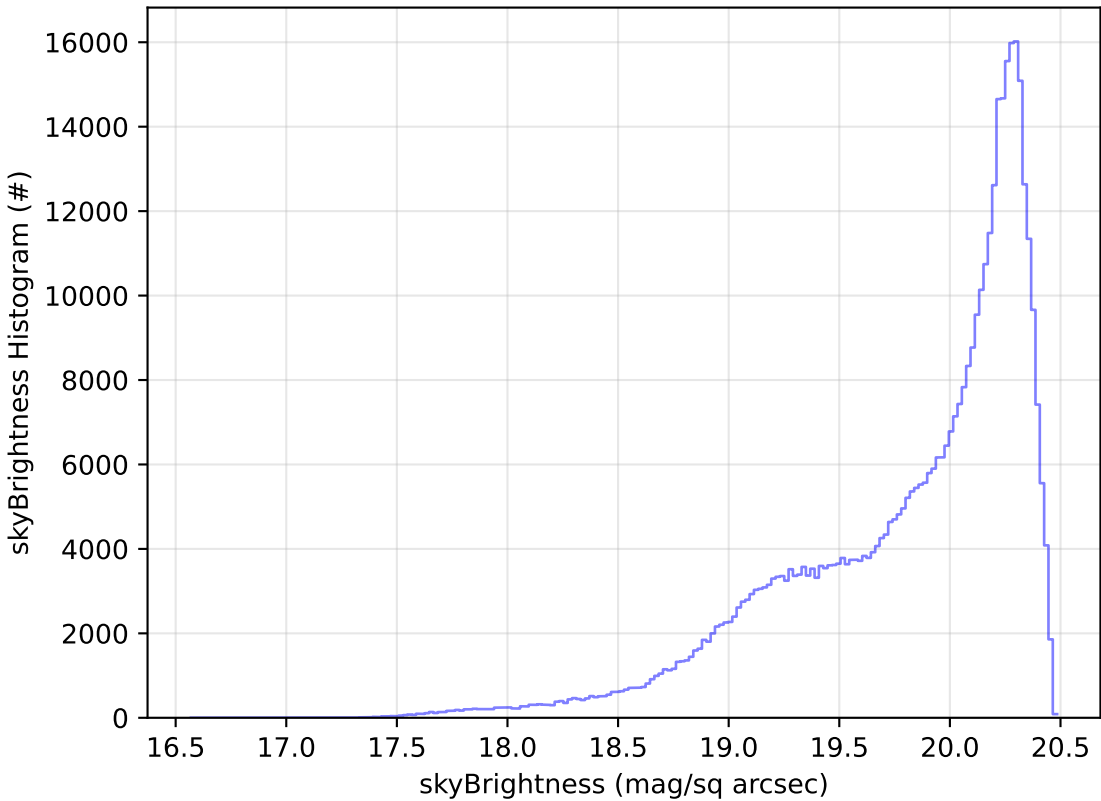
too_elab_r256_d2_ugrizy_v3.4_10yrs All sky i band: skyBrightness Histogram
