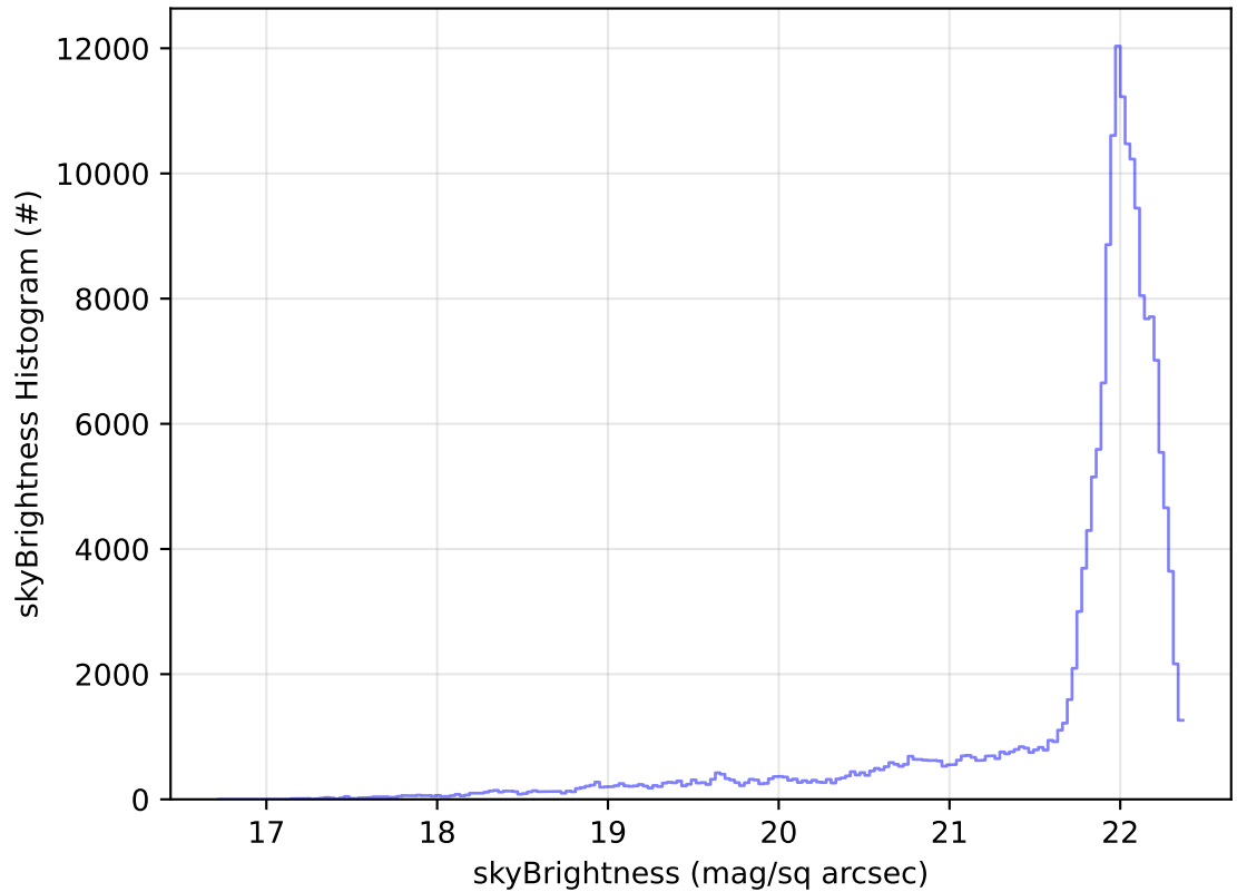
too_elab_r256_d2_ugrizy_v3.4_10yrs All sky g band: skyBrightness Histogram
