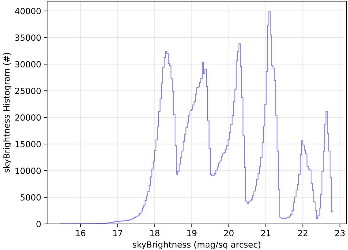
too_elab_r256_d2_ugrizy_v3.4_10yrs All sky all bands: skyBrightness Histogram
