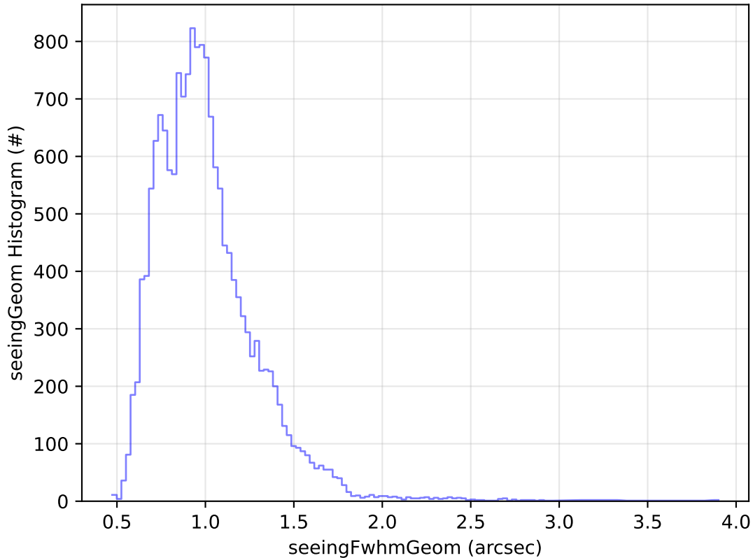
too_elab_r256_d2_ugrizy_v3.4_10yrs Yr 1 u band: seeingGeom Histogram
