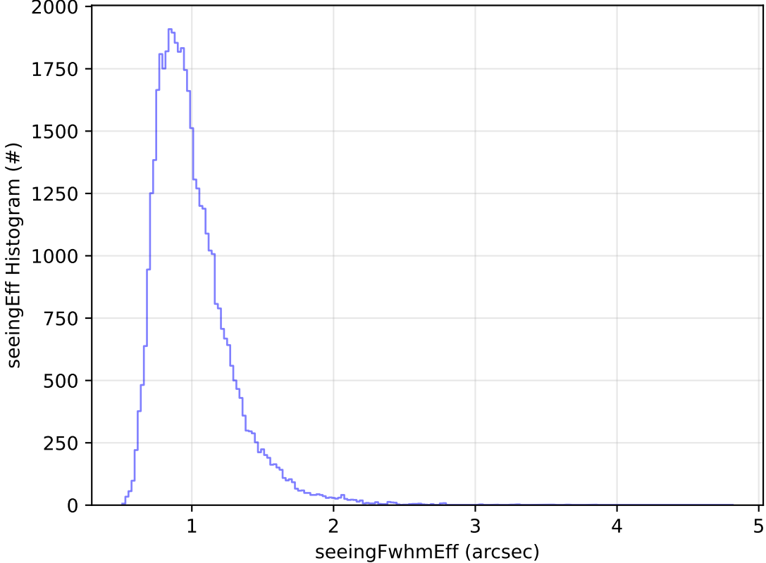
too_elab_r256_d2_ugrizy_v3.4_10yrs Yr 1 z band: seeingEff Histogram
