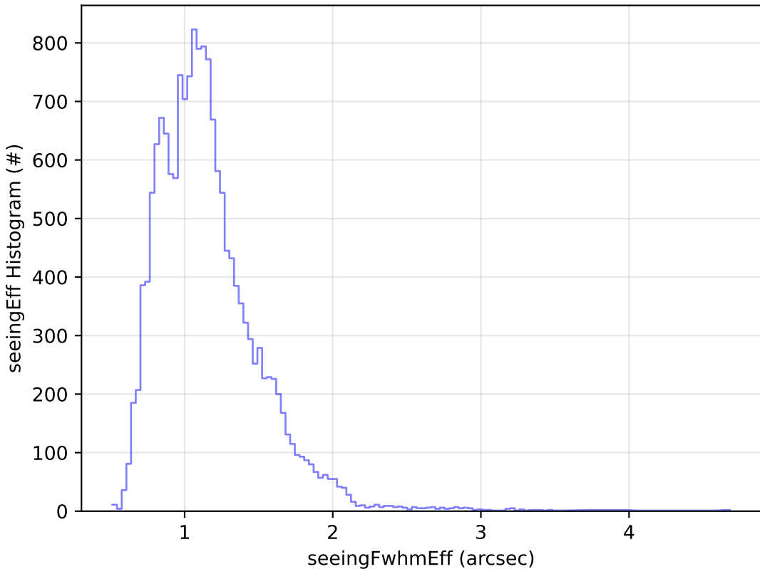
too_elab_r256_d2_ugrizy_v3.4_10yrs Yr 1 u band: seeingEff Histogram
