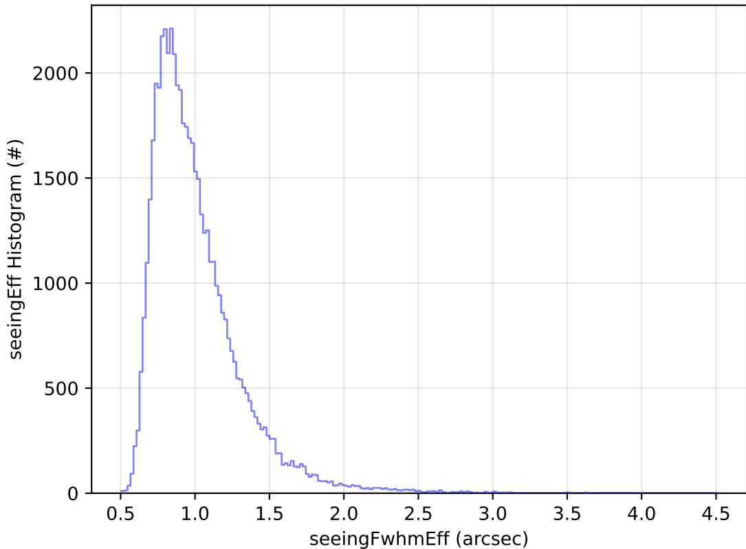
too_elab_r256_d2_ugrizy_v3.4_10yrs Yr 1 i band: seeingEff Histogram
