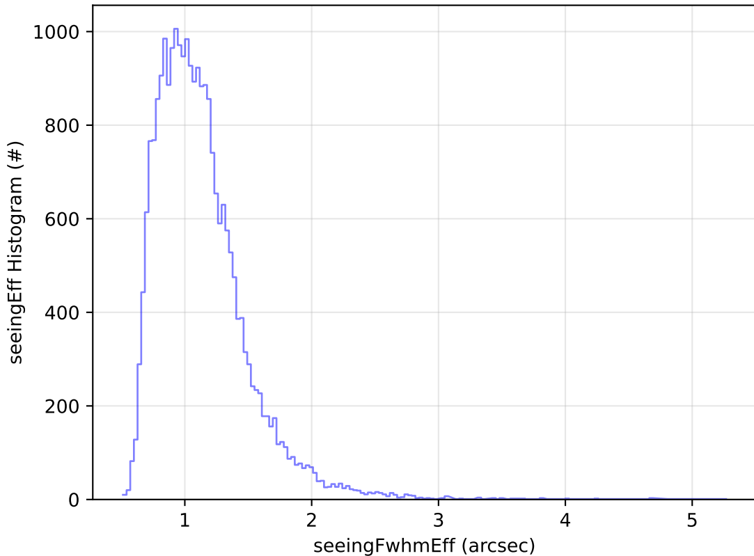
too_elab_r256_d2_ugrizy_v3.4_10yrs Yr 1 g band: seeingEff Histogram
