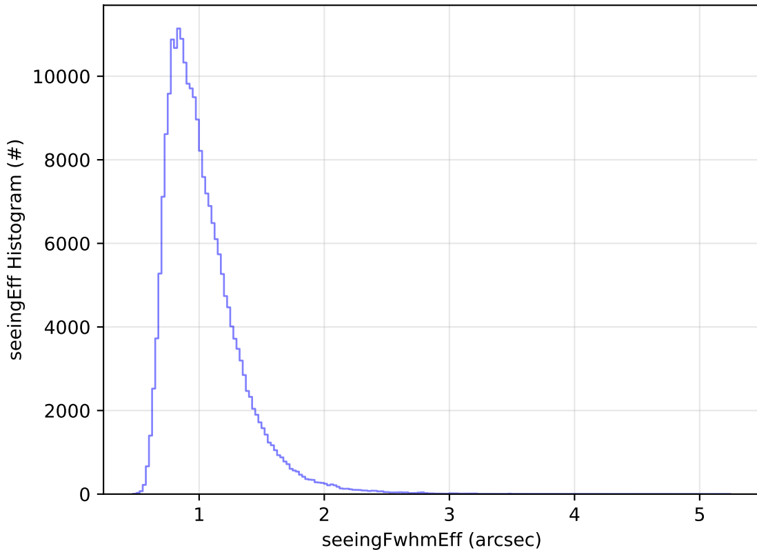
too_elab_r256_d2_ugrizy_v3.4_10yrs Yr 1 all bands: seeingEff Histogram
