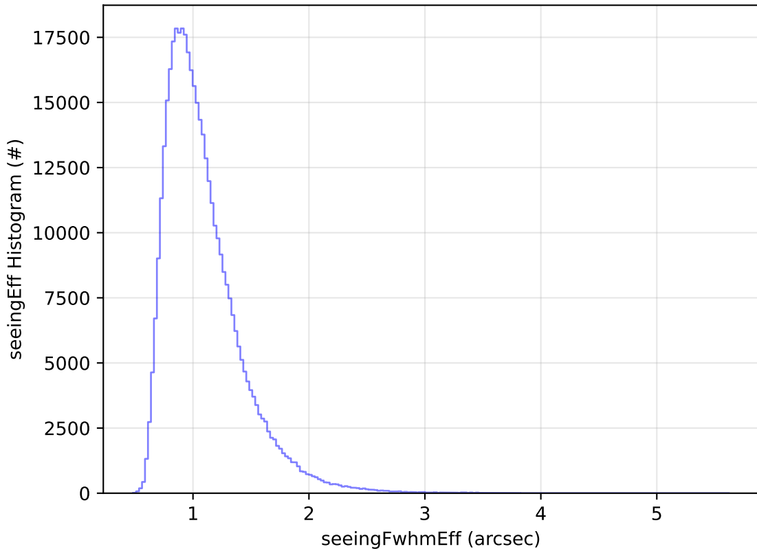
too_elab_r256_d2_ugrizy_v3.4_10yrs WFD z band: seeingEff Histogram
