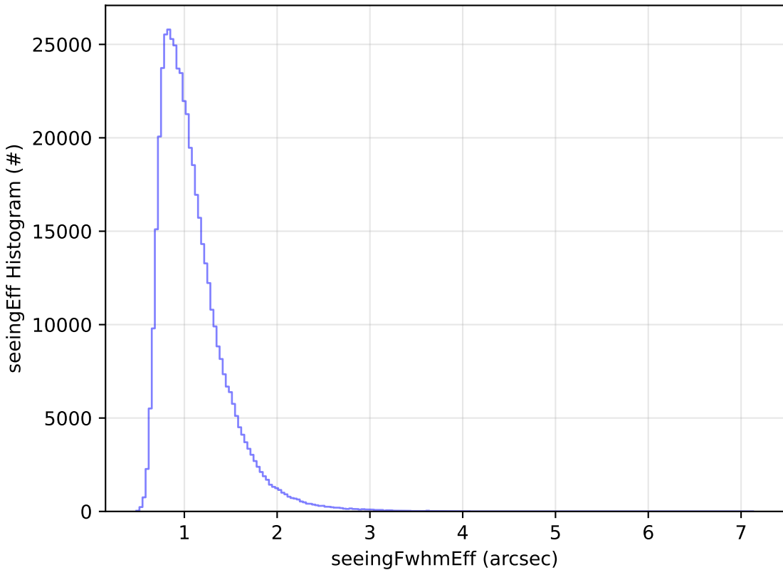
too_elab_r256_d2_ugrizy_v3.4_10yrs WFD i band: seeingEff Histogram
