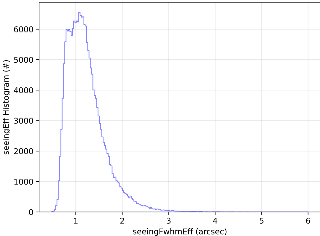
too_elab_r256_d2_ugrizy_v3.4_10yrs WFD g band: seeingEff Histogram
