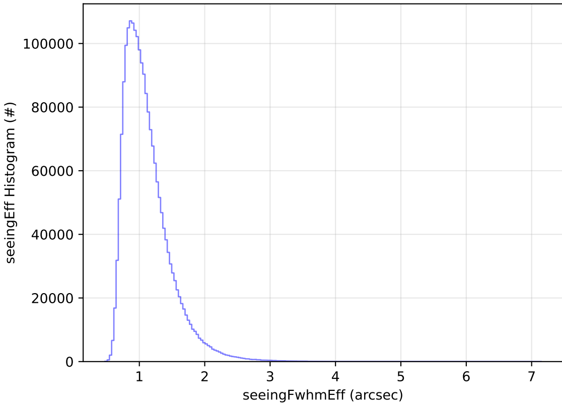
too_elab_r256_d2_ugrizy_v3.4_10yrs WFD all bands: seeingEff Histogram
