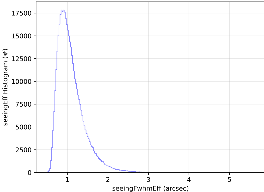
too_elab_r256_d2_ugrizy_v3.4_10yrs All sky z band: seeingEff Histogram
