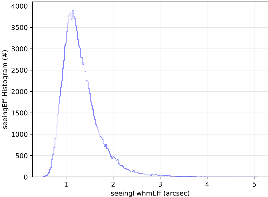
too_elab_r256_d2_ugrizy_v3.4_10yrs All sky u band: seeingEff Histogram
