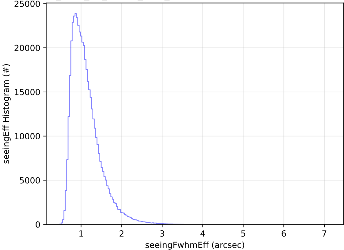
too_elab_r256_d2_ugrizy_v3.4_10yrs All sky r band: seeingEff Histogram
