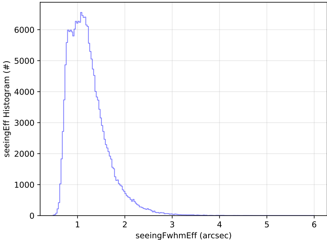
too_elab_r256_d2_ugrizy_v3.4_10yrs All sky g band: seeingEff Histogram
