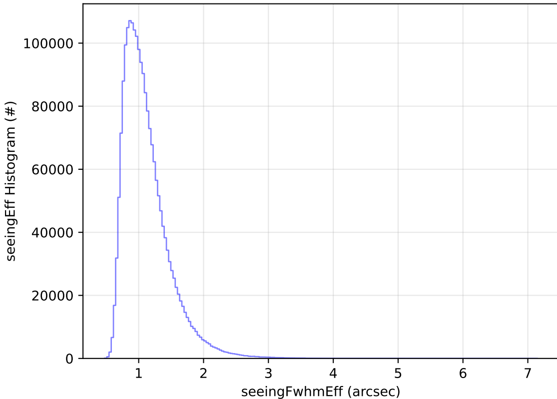
too_elab_r256_d2_ugrizy_v3.4_10yrs All sky all bands: seeingEff Histogram
