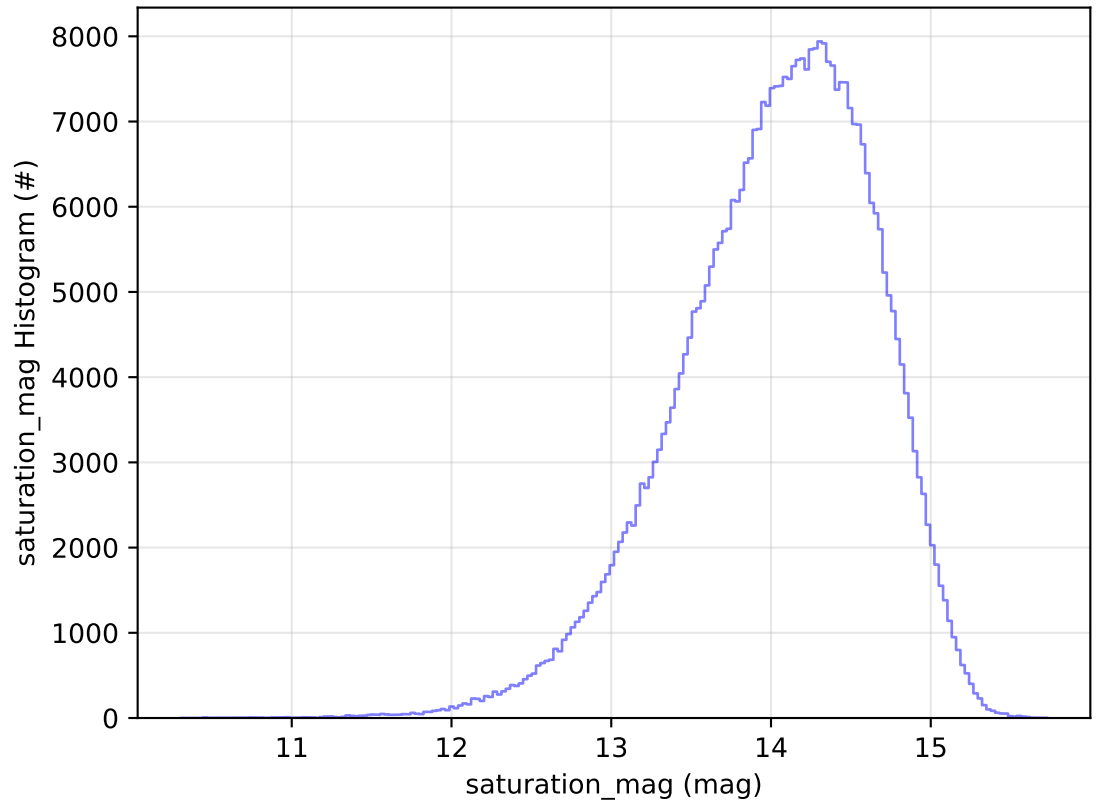
too_elab_r256_d2_ugrizy_v3.4_10yrs WFD z band: saturation_mag Histogram
