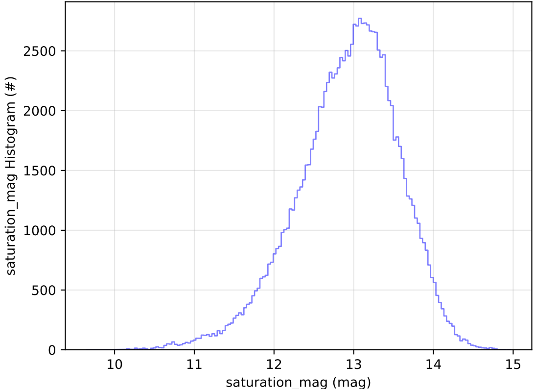
too_elab_r256_d2_ugrizy_v3.4_10yrs WFD u band: saturation_mag Histogram
