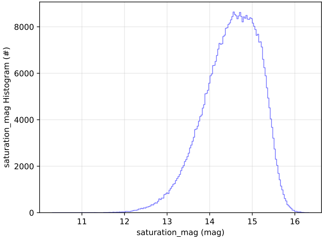
too_elab_r256_d2_ugrizy_v3.4_10yrs WFD r band: saturation_mag Histogram
