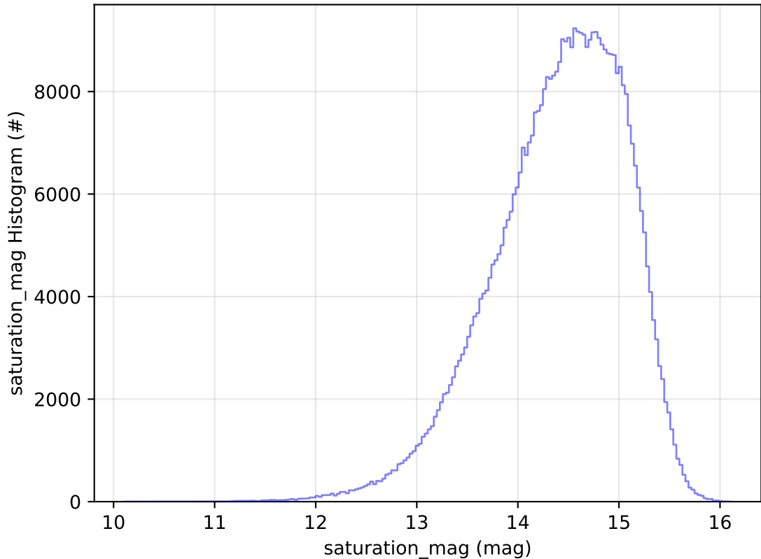
too_elab_r256_d2_ugrizy_v3.4_10yrs WFD i band: saturation_mag Histogram
