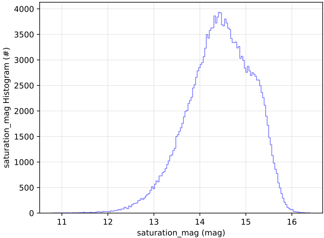
too_elab_r256_d2_ugrizy_v3.4_10yrs WFD g band: saturation_mag Histogram
